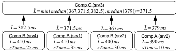
Fig. 3. Propagation of SLA from parents to children. The child Comp C receives 4 SLA updates from its parents: 3 from replicas of Comp B and 1 from Comp A . The new SLA of the child component is computed following equation (10).
